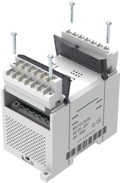
Plug-in screw terminals:
