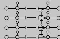
MRK TEST - 10 4 Poles Test Disconnect Set New Code: 1010229 Old Code: 1305
